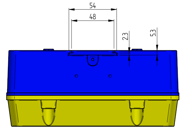
VIEW ON SLOT SCALE: 1:2.5
