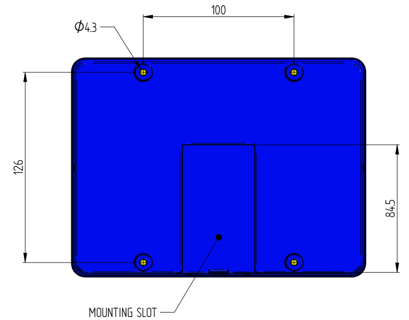
VIEW ON REAR SCALE: 1:2.5
